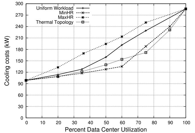
Fig. 6. Cooling costs for our three baseline algorithms and our thermal-topology-based algorithm. The Weatherman-based workload placement algorithm achieves savings comparable to the previous best in temperature-aware workload placement.
