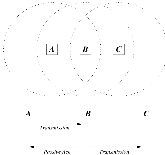
Fig. 8. Passive acknowledgments.
