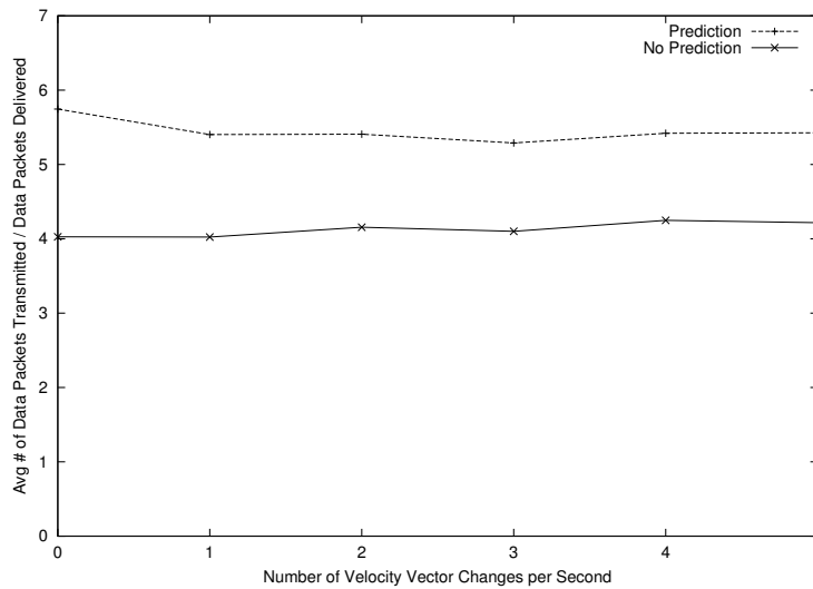
Fig. 26. Average number of data packets transmitted per data packet delivered as a function of direction changing frequency.
