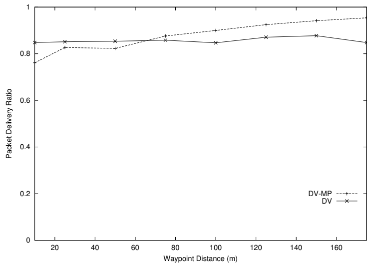
Fig. 29. Packet delivery ratio as a function of waypoint distance.
