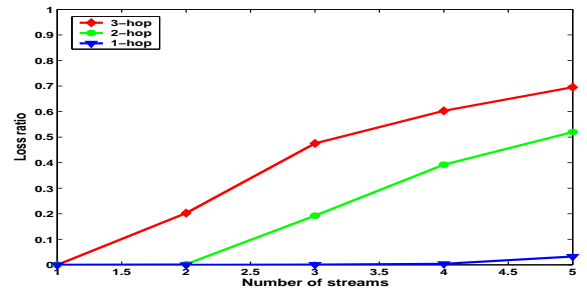
(b) Loss.
