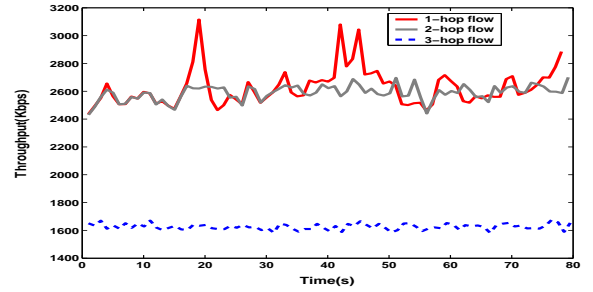
(a) Throughput.
