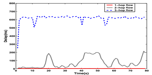
(c) Delay.
