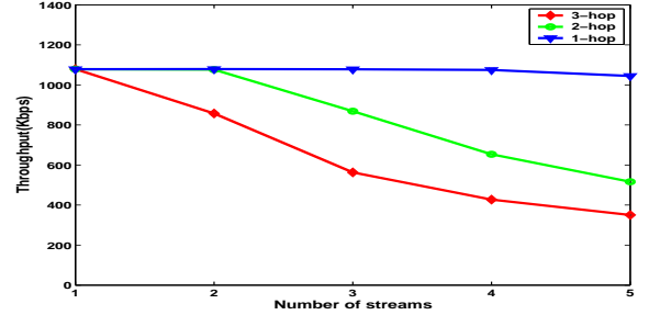
(a) Throughput.
