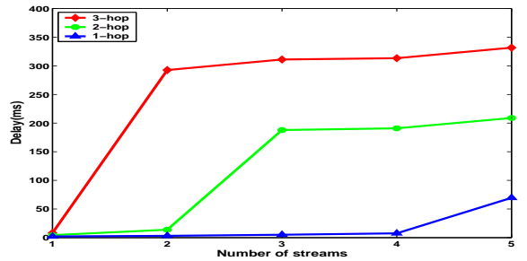
(c) Delay.
