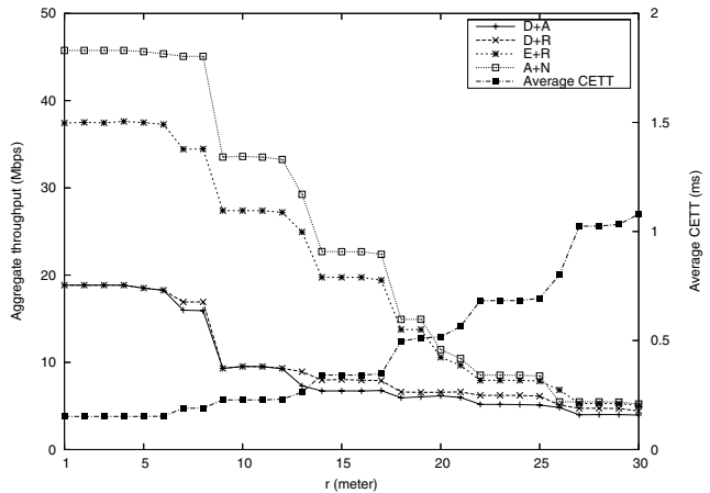
Fig. 4. Aggregate throughput in three-node ( N = 3 ) chain topology networks with varying link distance ( r ).
