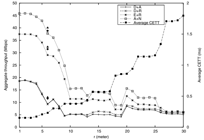
Fig. 6. Aggregate throughput in five-node ( N = 5 ) chain topology networks with varying link distance ( r ).
