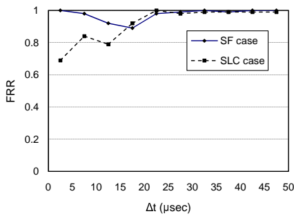
Figure 4: FRR vs. arrival time difference \Delta t for SF and SLC cases. \Delta t is defined as “the arrival time of the interferer’s frame minus the arrival time of the sender’s frame.”
