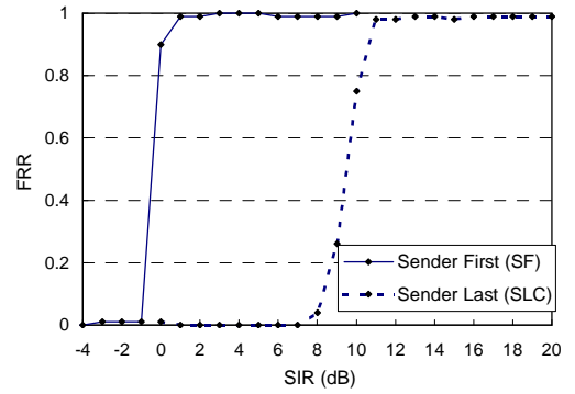
Figure 5: FRR vs. SIR with 6Mbps sender/interferer’s transmissions. SIR is defined as “RSS from sender minus RSS from interferer.”
