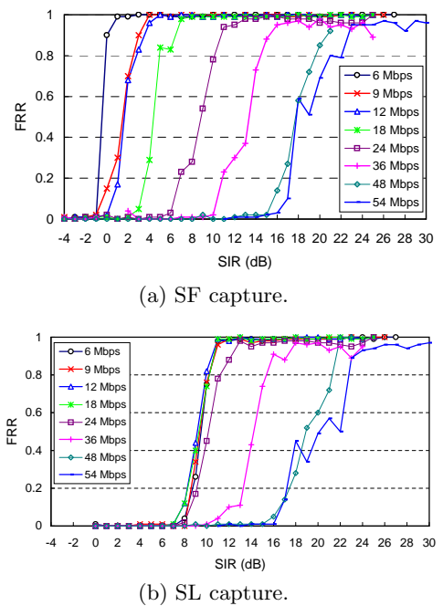
Figure 7: Sender's PHY rate changes while the interferer's PHY rate is fixed at 6Mbps.
