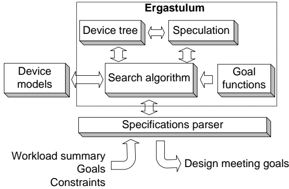
Figure 1: Ergastulum’s architecture: The search algorithm uses the device tree to keep track of the current design, and the speculation engine to rapidly switch between alternative designs. Different goal functions are used in different phases of the search. Ergastulum takes its input (and generates its output) in the Rome specification language [34]. The device models are used to quantitatively evaluate the quality of the design.
