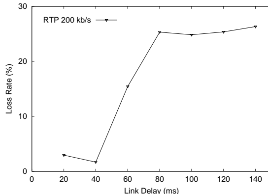
Fig. 15. Effect of link latency variation on RTP stream loss rate.
