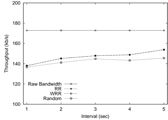
Fig. 6. TCP throughput as a function of up-time interval.
