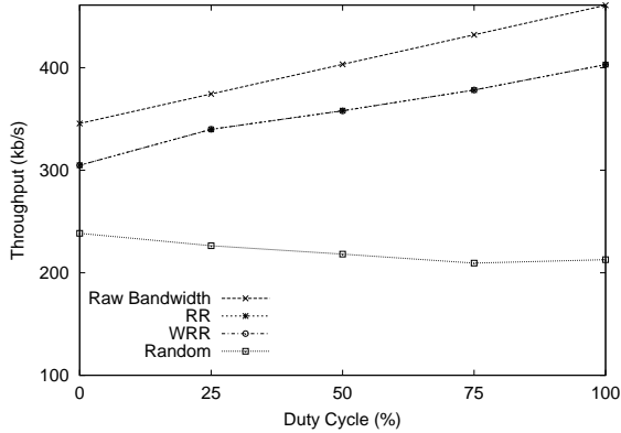
Fig. 4. TCP throughput with 3 persistent links and 1 transient link.
