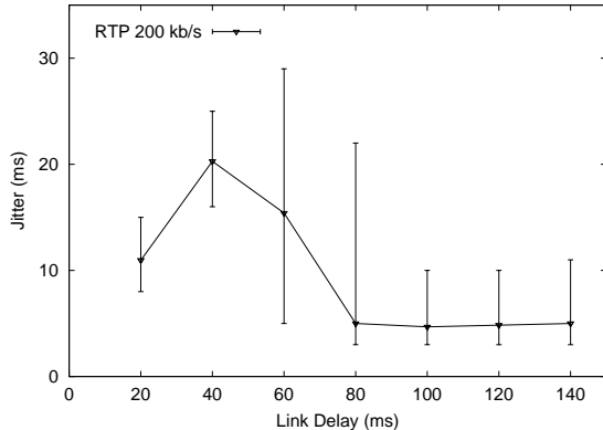
Fig. 16. Effect of link latency variation on RTP stream jitter.
