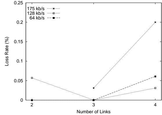
Fig. 13. Effect of piconet size on RTP stream loss rate.
