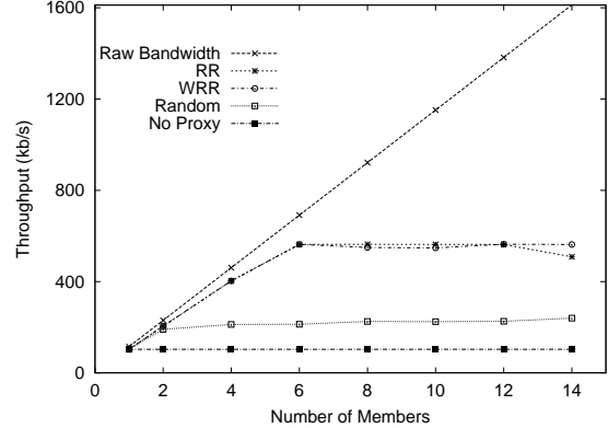
Fig. 3. TCP throughput as a function of piconet size.
