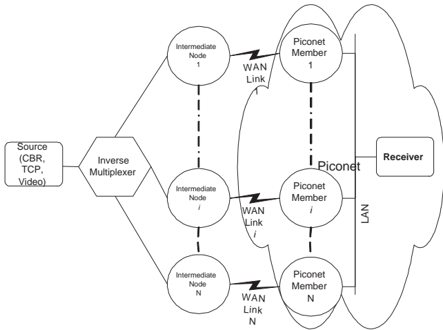
Fig. 2. Simulation topology.
