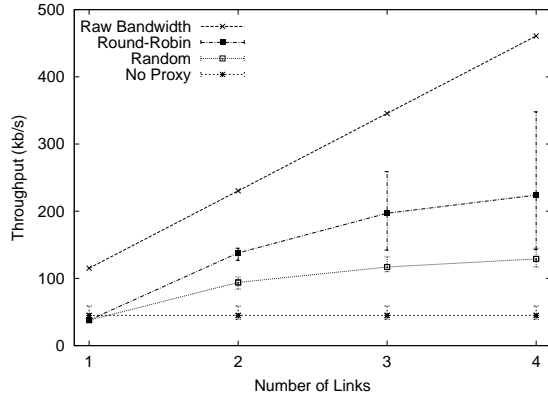
Fig. 10. Effect of piconet size on TCP throughput.
