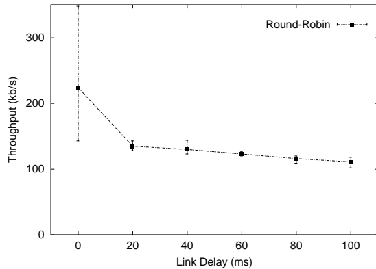
Fig. 11. Effect of link latency variation on TCP throughput.
