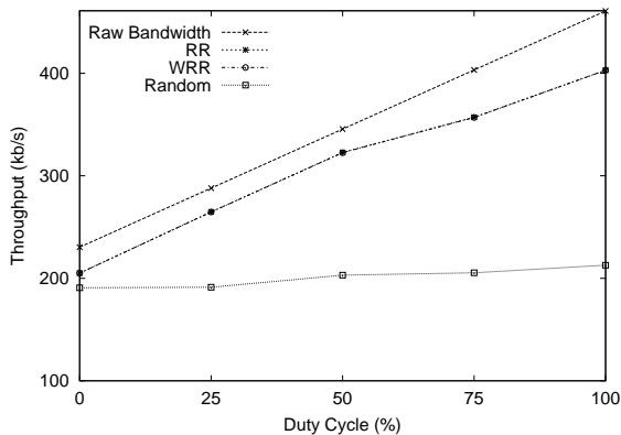
Fig. 5. TCP throughput with 2 persistent links and 2 transient links.
