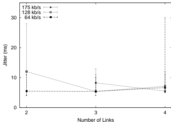
Fig. 14. Effect of piconet size on RTP stream jitter.
