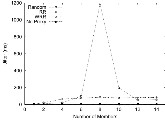
Fig. 7. CBR jitter as a function of piconet size.
