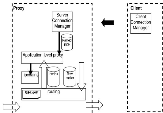
Fig. 8. Linux-based implementation of an aggregation proxy.
