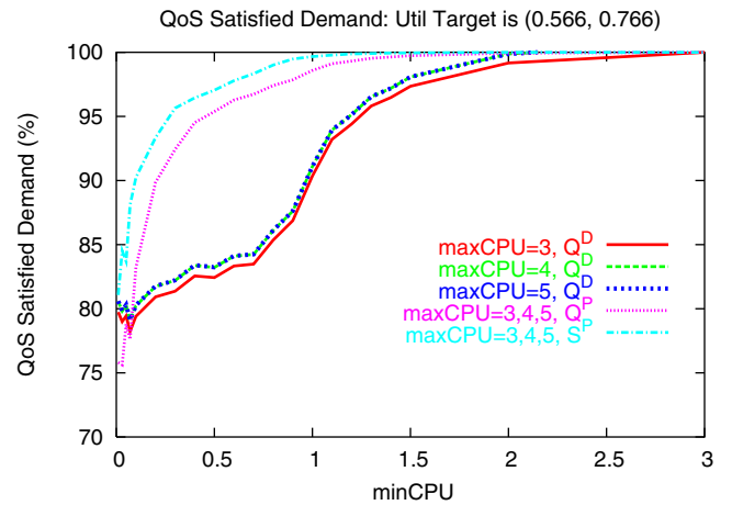
Fig. 17. Fast Allocation Policy : minCPU requirements v.s. service metrics Q^D , Q^P , and S^P for Low QoS
