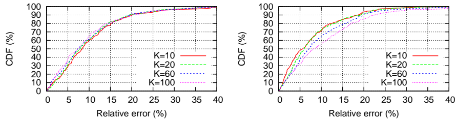
Fig. 12: Server 1. CDF of relative errors under a different number of of core transactions chosen for a regression method: (a) training set, (b) validating set.
