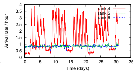
(b) Top 4-6 transactions
