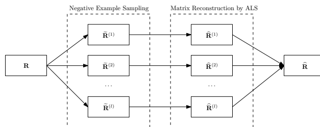
Figure 1: A diagram that illustrates an ensemble based on negative exempling sampling for OCCF
