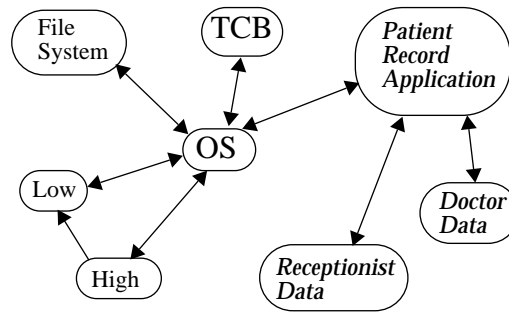
Non-hierarchical Security
