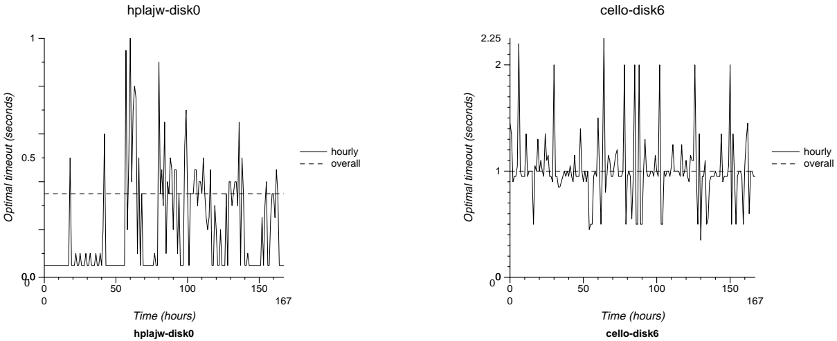
Figure 17: optimal fixed timeout values for two traces.
