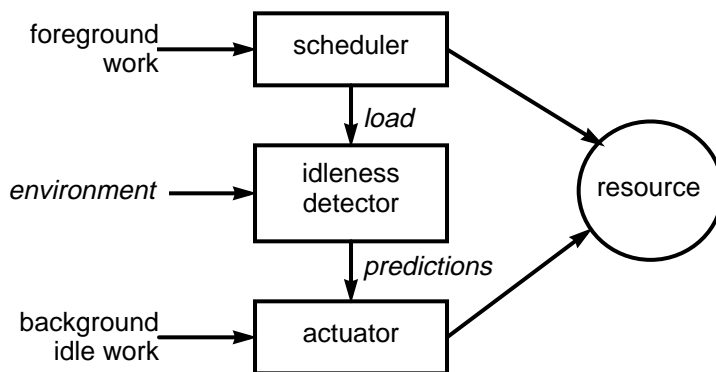
Figure 1: the idle-time processing framework.
