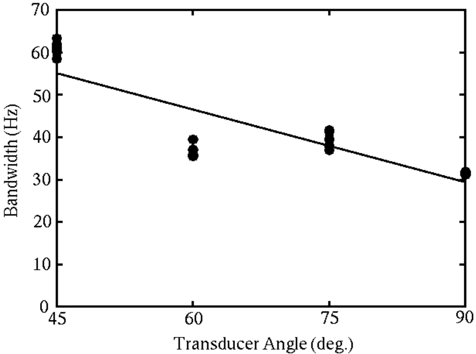
Figure 10: Bandwidth versus transducer angle for real flow. Flow velocity = 12 cm/s; two-way pulse length = 0.6 mm.
