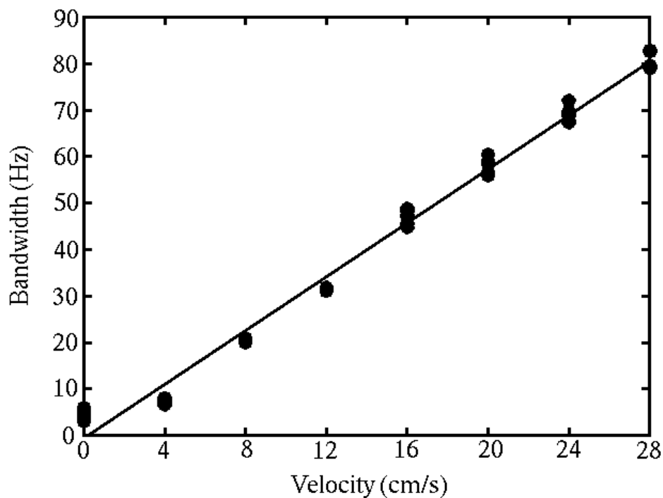
Figure 8: Bandwidth versus velocity for real flow (bandwidths were estimated with DC components removed from the power spectra). Transducer angle = 90°; two-way pulse length = 0.6 mm.
