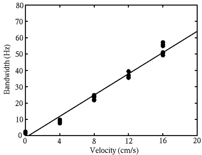
Figure 4: Bandwidth versus velocity for real flow. Transducer angle = 60°; two-way pulse length = 0.6 mm.
