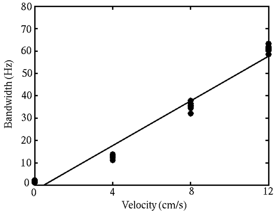
Figure 5: Bandwidth versus velocity for real flow. Transducer angle = 45°; two-way pulse length = 0.6 mm.
