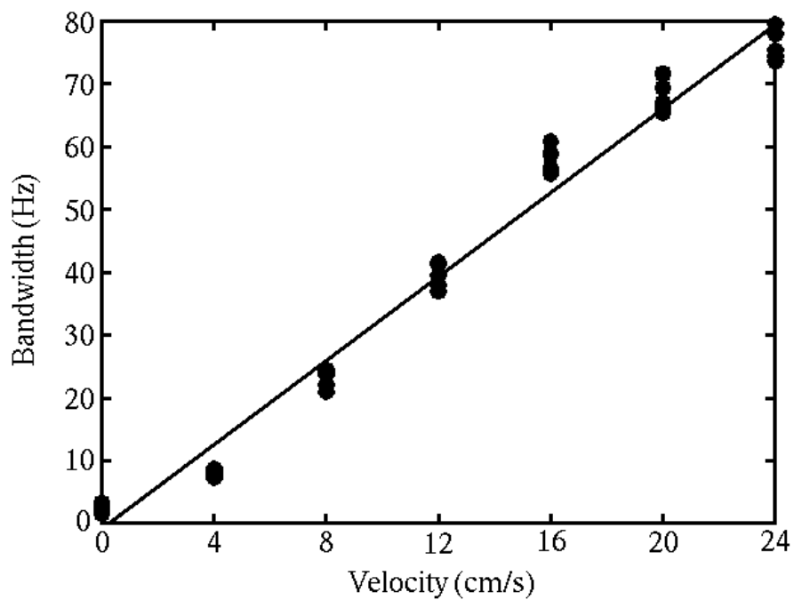
Figure 6: Bandwidth versus velocity for real flow. Transducer angle = 75°; two-way pulse length = 0.6 mm.
