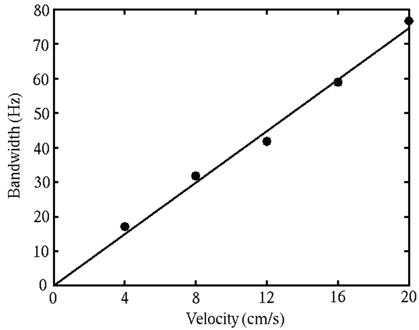
Figure 3: Bandwidth versus velocity for ideal uniform flow. Transducer angle = 60°; two-way pulse length = 0.6 mm.
