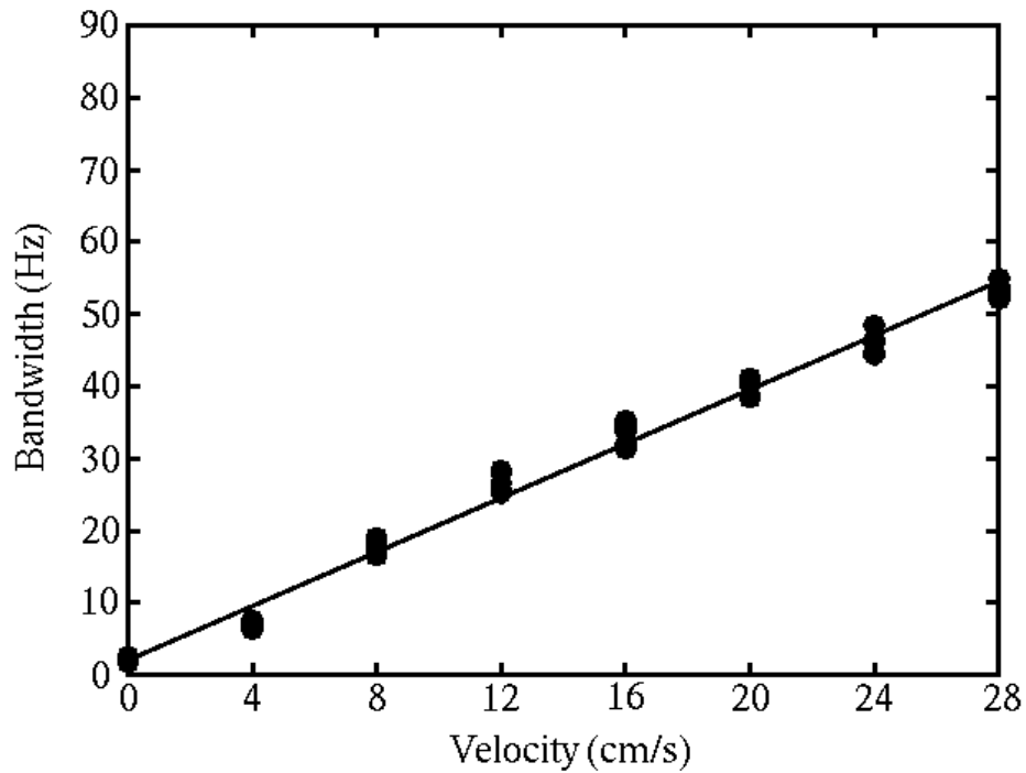
Figure 7: Bandwidth versus velocity for real flow (bandwidths were estimated with DC components in the power spectra). Transducer angle = 90°; two-way pulse length = 0.6 mm.
