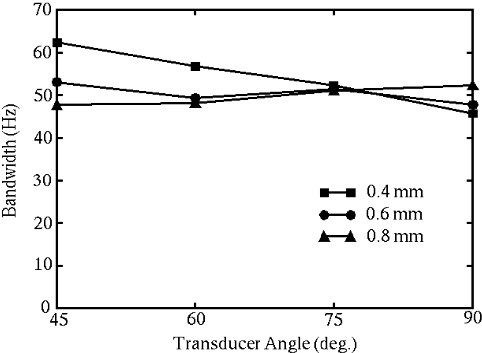
Figure 9: Bandwidth versus transducer angle for ideal uniform flow. Flow velocity = 12 cm/s; two-way pulse lengths = 0.4, 0.6, 0.8 mm.
