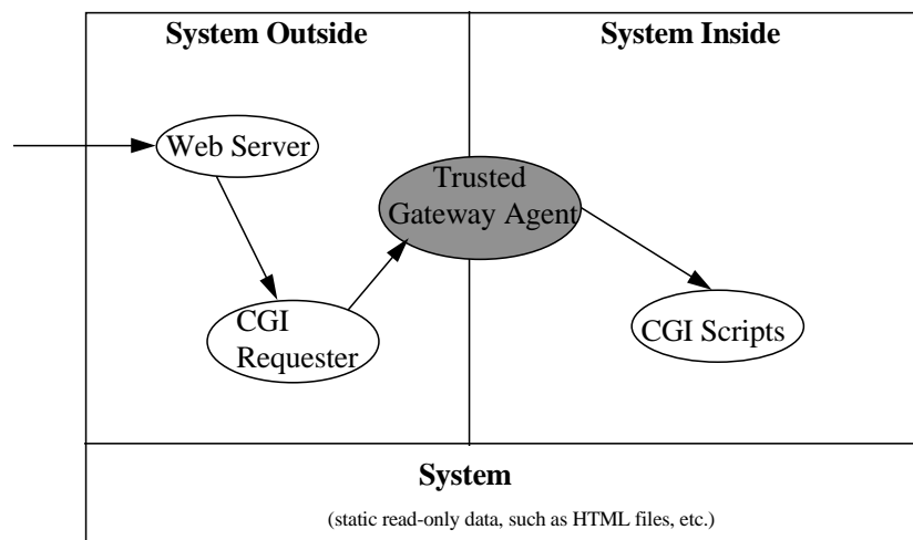
Figure 2: VirtualVault Architecture
