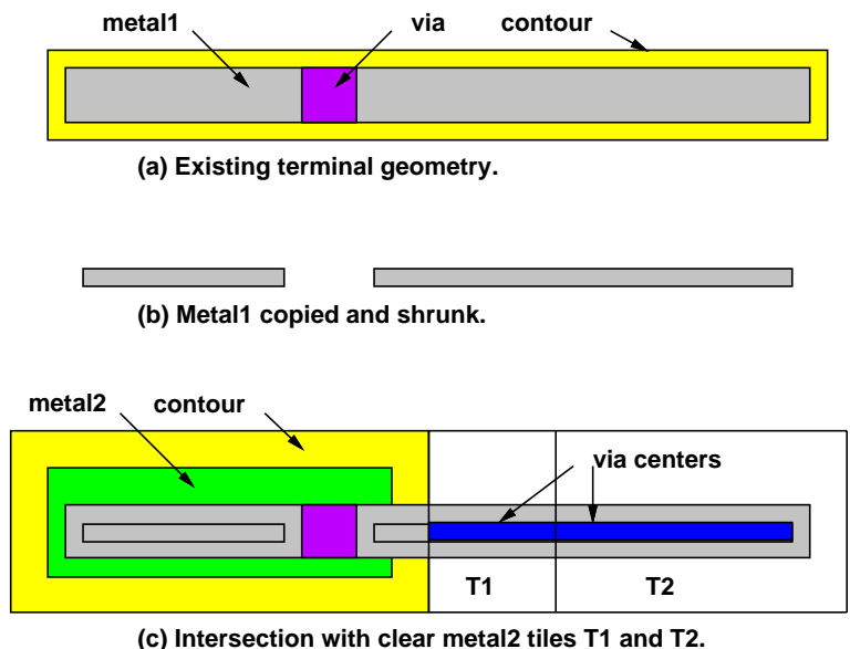
Figure 5: Starting With a Via
